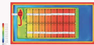
Thermal simulation diagram of the pack
